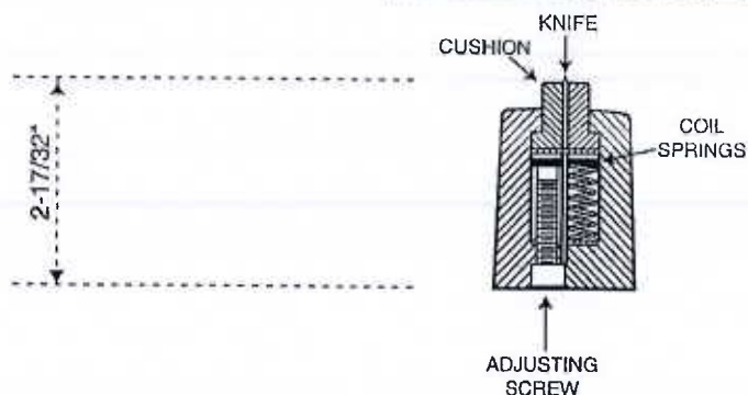
SINGLE WIDTH KNIFE BOX ASSEMBLY SC, SSC & SUBURBAN
