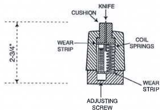
3:2 KNIFE BOX ASSEMBLY
